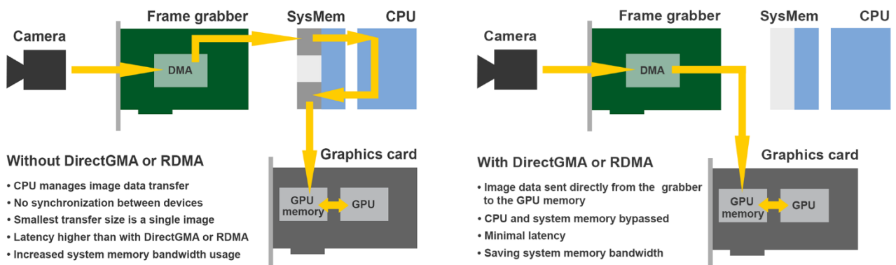
Figure 2: GPU Access – traditional versus using AMD's DirectGMA
