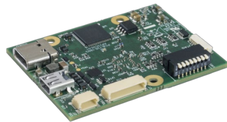
Figure 2. Reverse side of Harrier USB/HDMI Camera Interface Board
