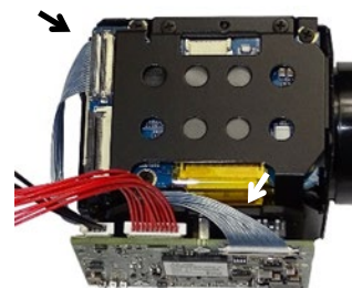
Figure 8. KEL cable connects the interface board to the Harrier 10x AF-Zoom Camera
