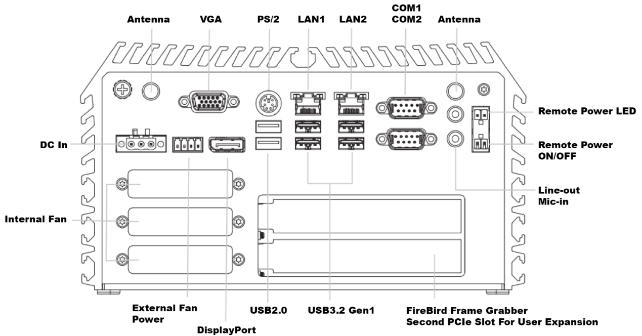
Figure 2. Oncilla 1402 Industrial PC Rear View.
