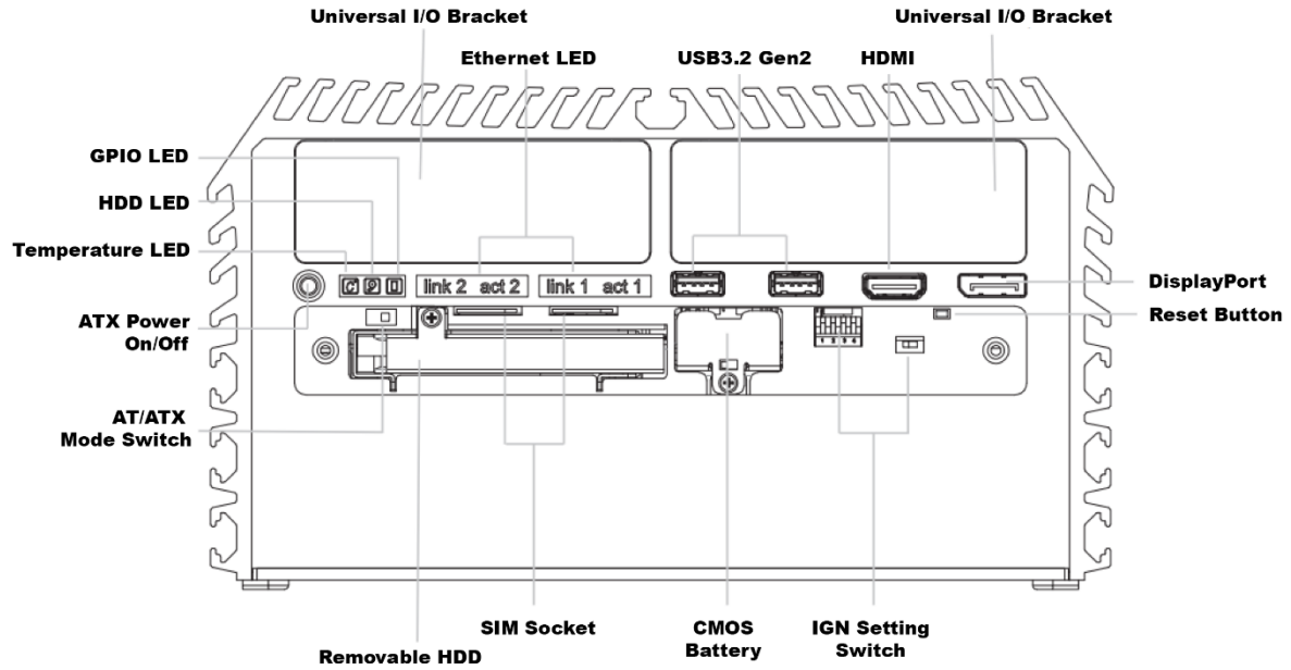
Figure 1. Oncilla 1402 Industrial PC Front View with HDD Panel Removed.
