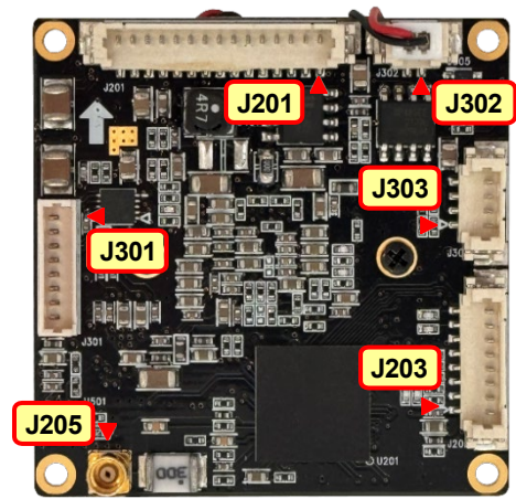
Bottom/Rear View
